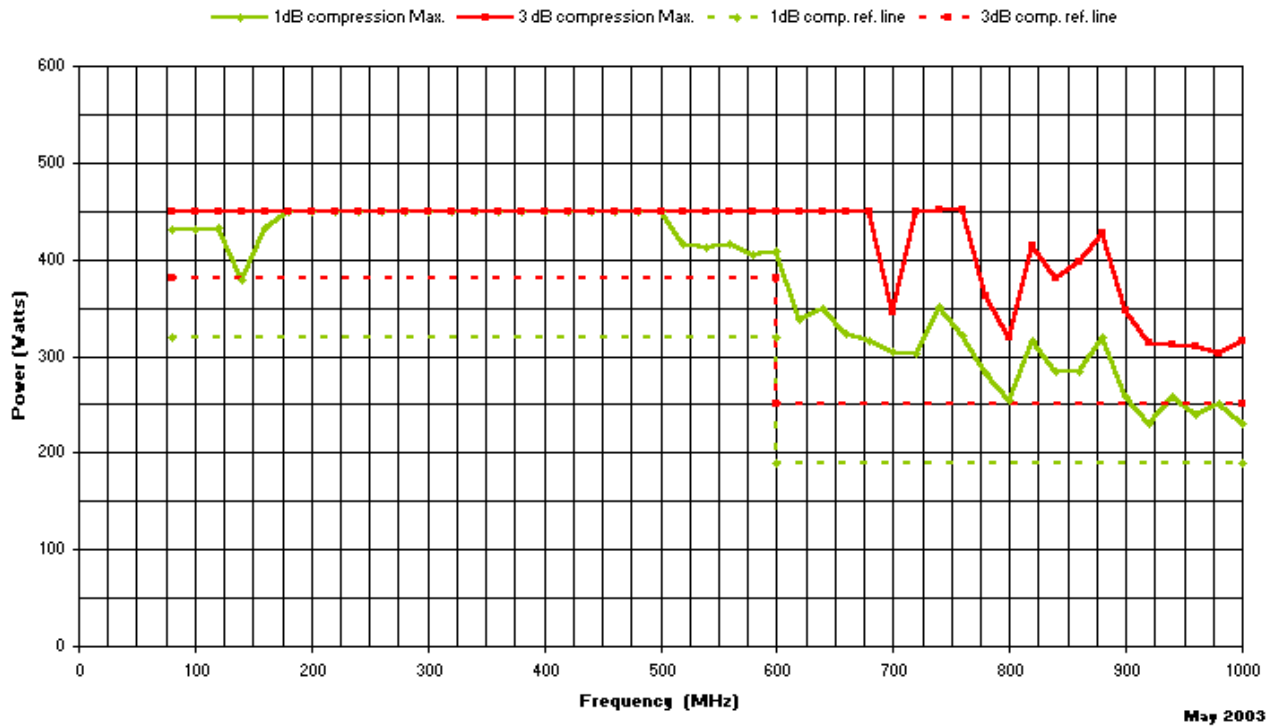
AP32 MT230 POWER AMPLIFIER - 300W / 80MHz - 1000MHz - Typical Power
