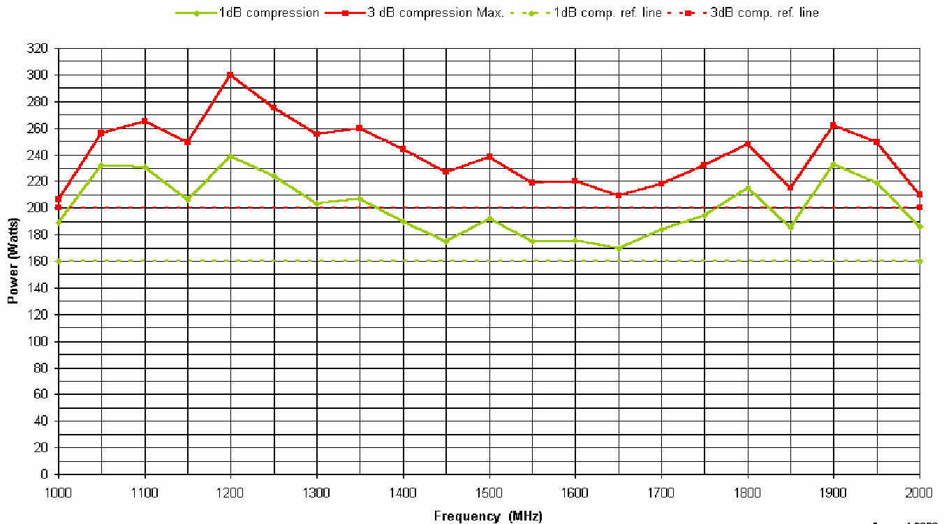
AP32 TU220 POWER AMPLIFIER - 200W / 1GHz - 2GHz - Typical Power
